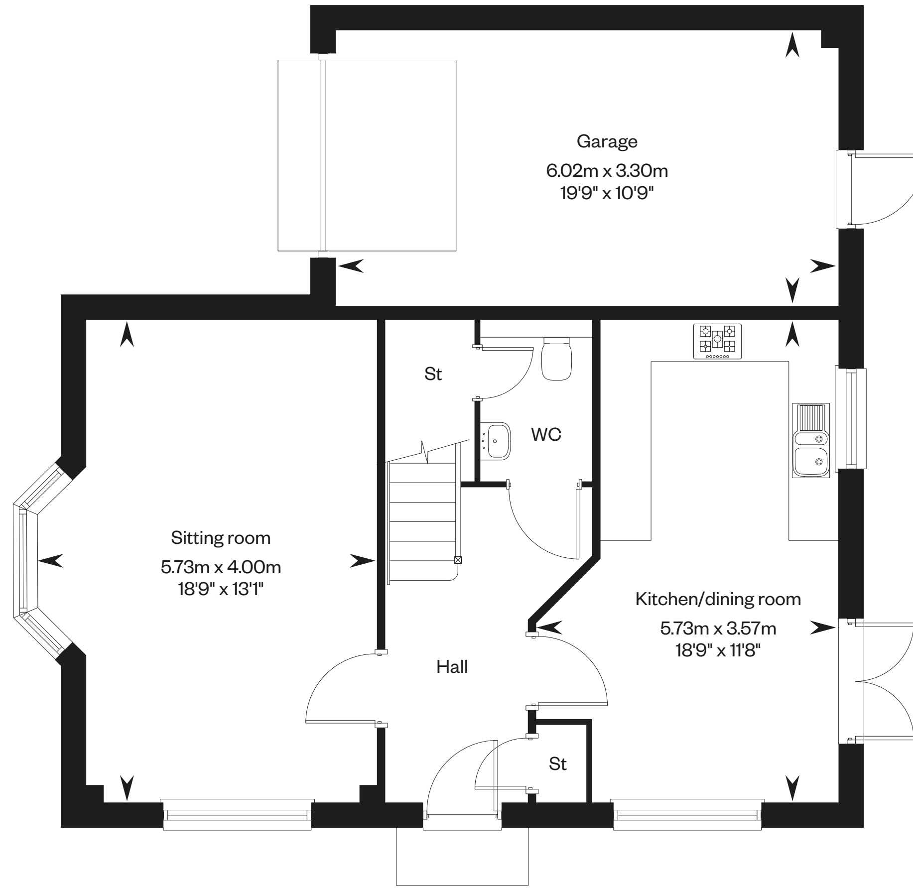
Ground floor
