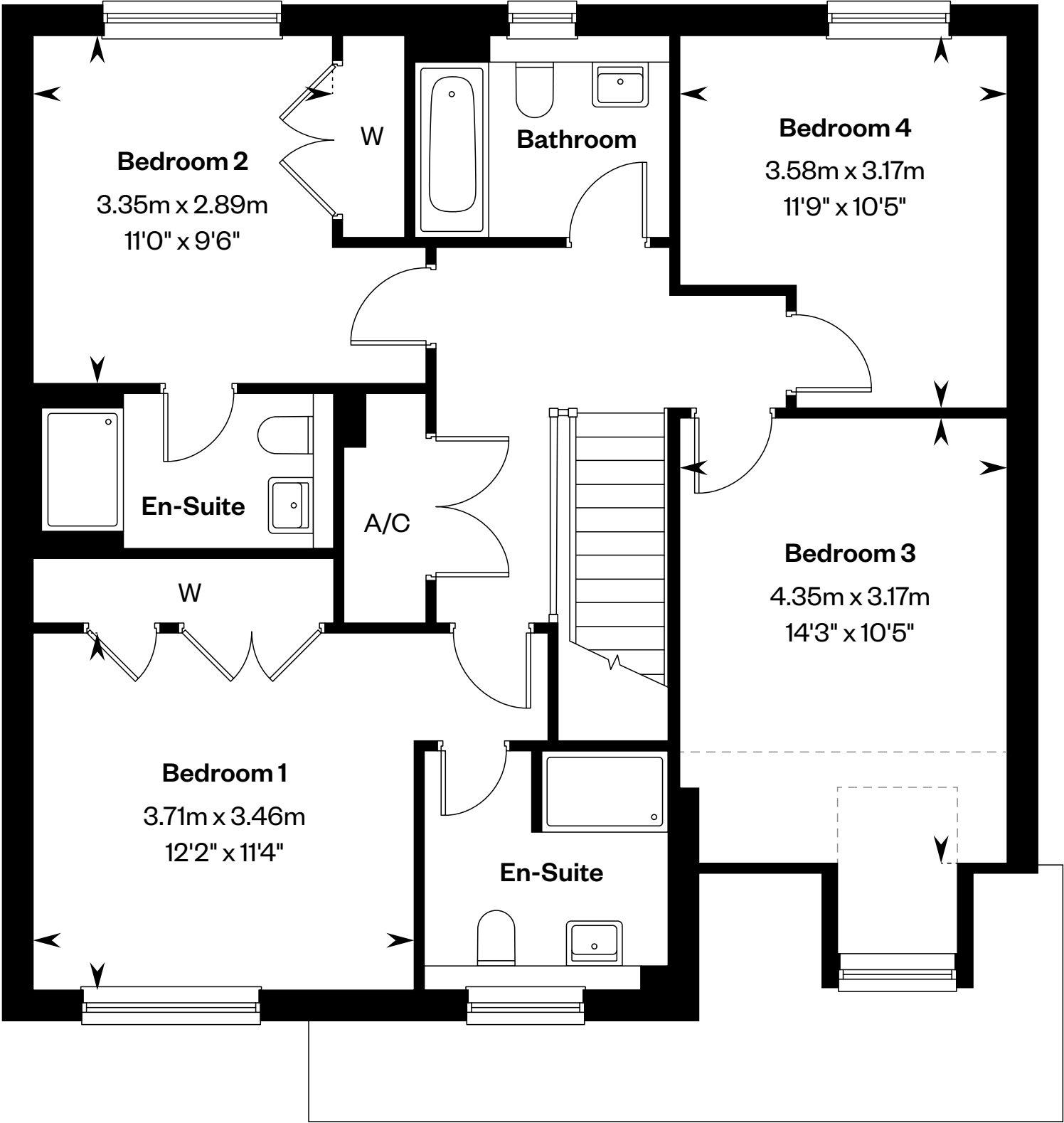
First floor
