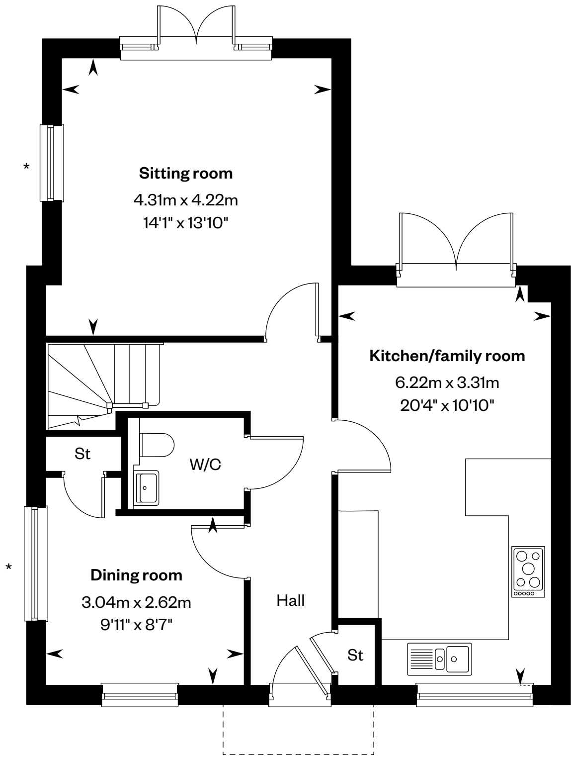
Ground floor
