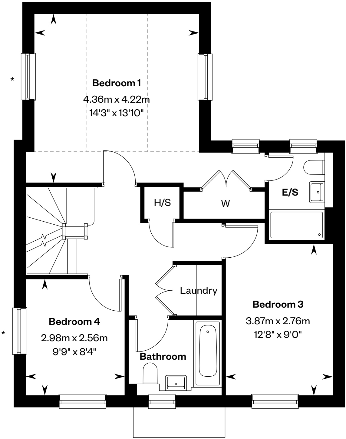
First floor
